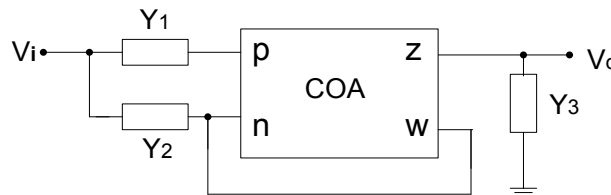
Figure 3. Proposed circuit topology
