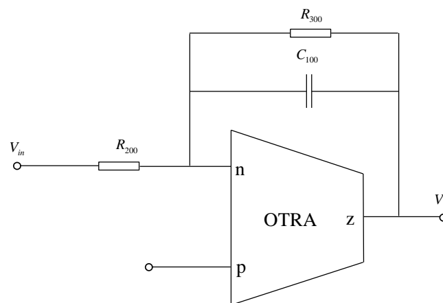
Figure 6 Voltage mode first order Lowpass filter
