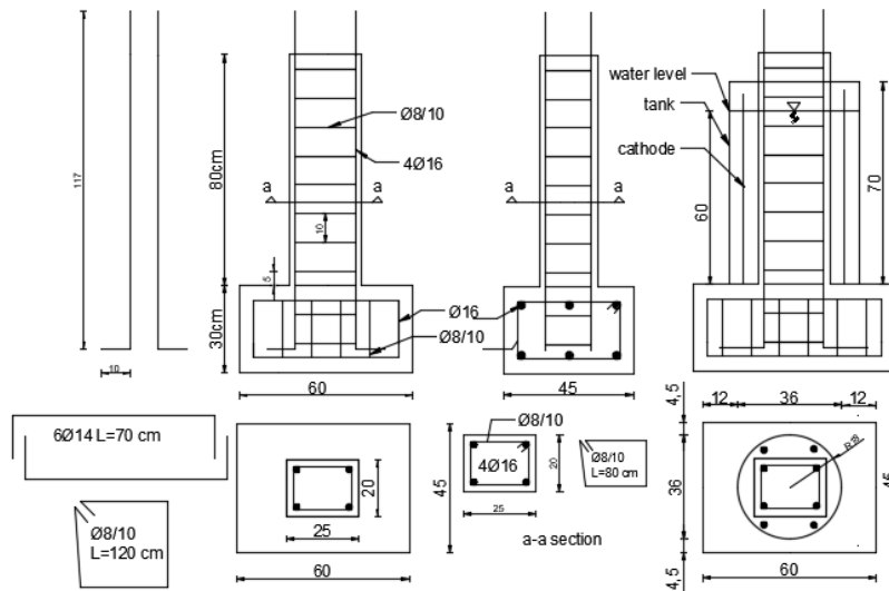
Figure 1. Specimen Detail
