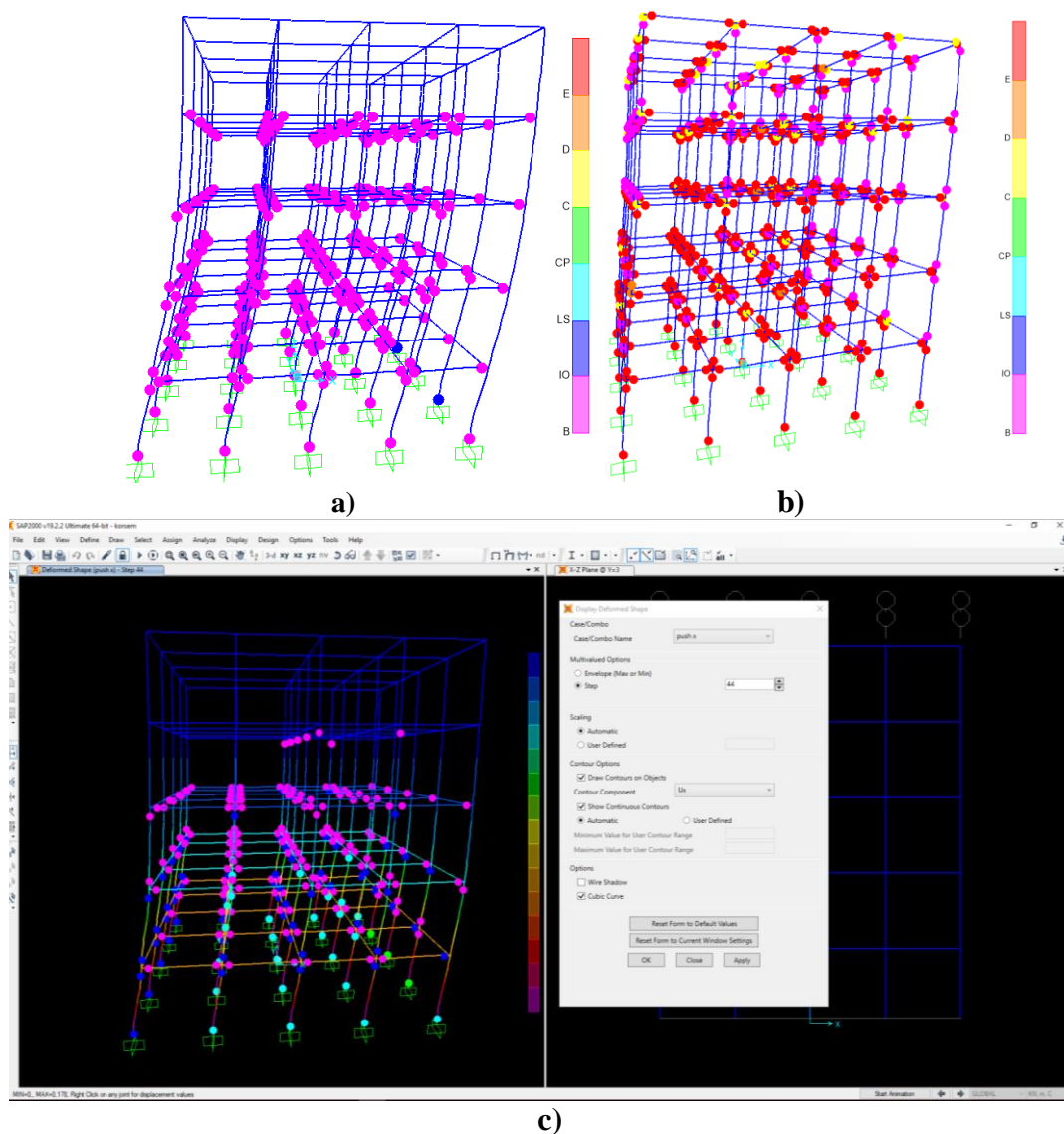
Figure 8. a) Development of plastic hinges in beams, b) Development plastic hinge in columns, c) Hinge status in reference building.
