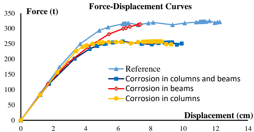
Figure 7. Load-displacement curves of all scenarios
