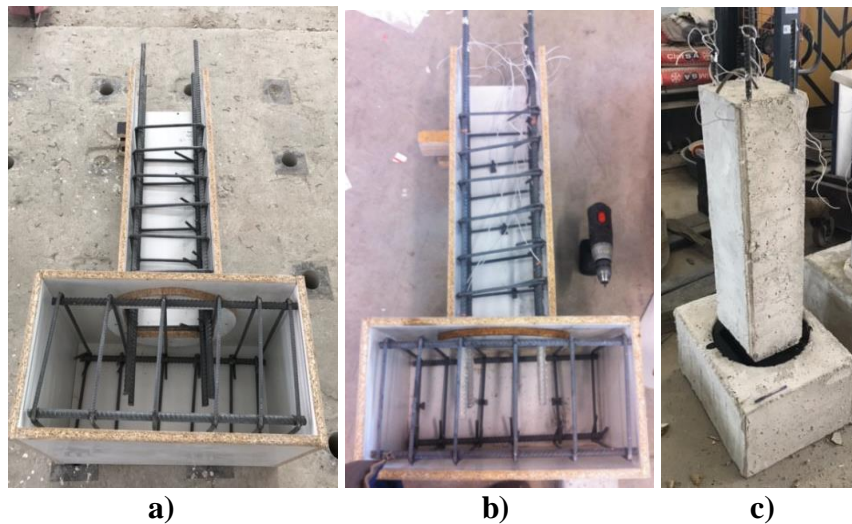
Figure 2. a) Sample mold plan, b) Insulation of sample, c) Insulation of anchor rods with epoxy resin.
