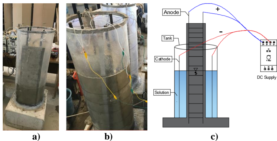
Figure 2. a) Preparing the tank and fixing it on the foundation, b) Filling with NaCl solution, c) Electrolysis cell diagram of specimen.
