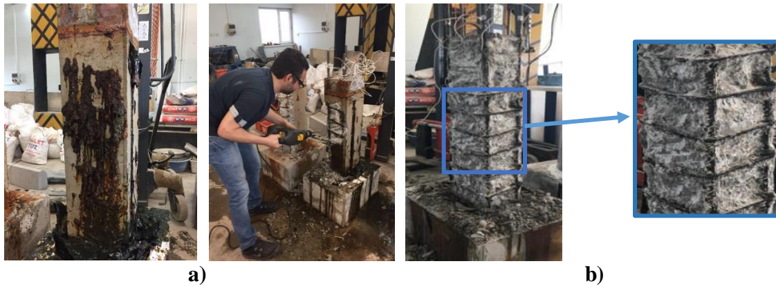
Figure 3. a) View of samples after the experiment, b) Peeling of concrete covers and corrosion distribution of specimen.
